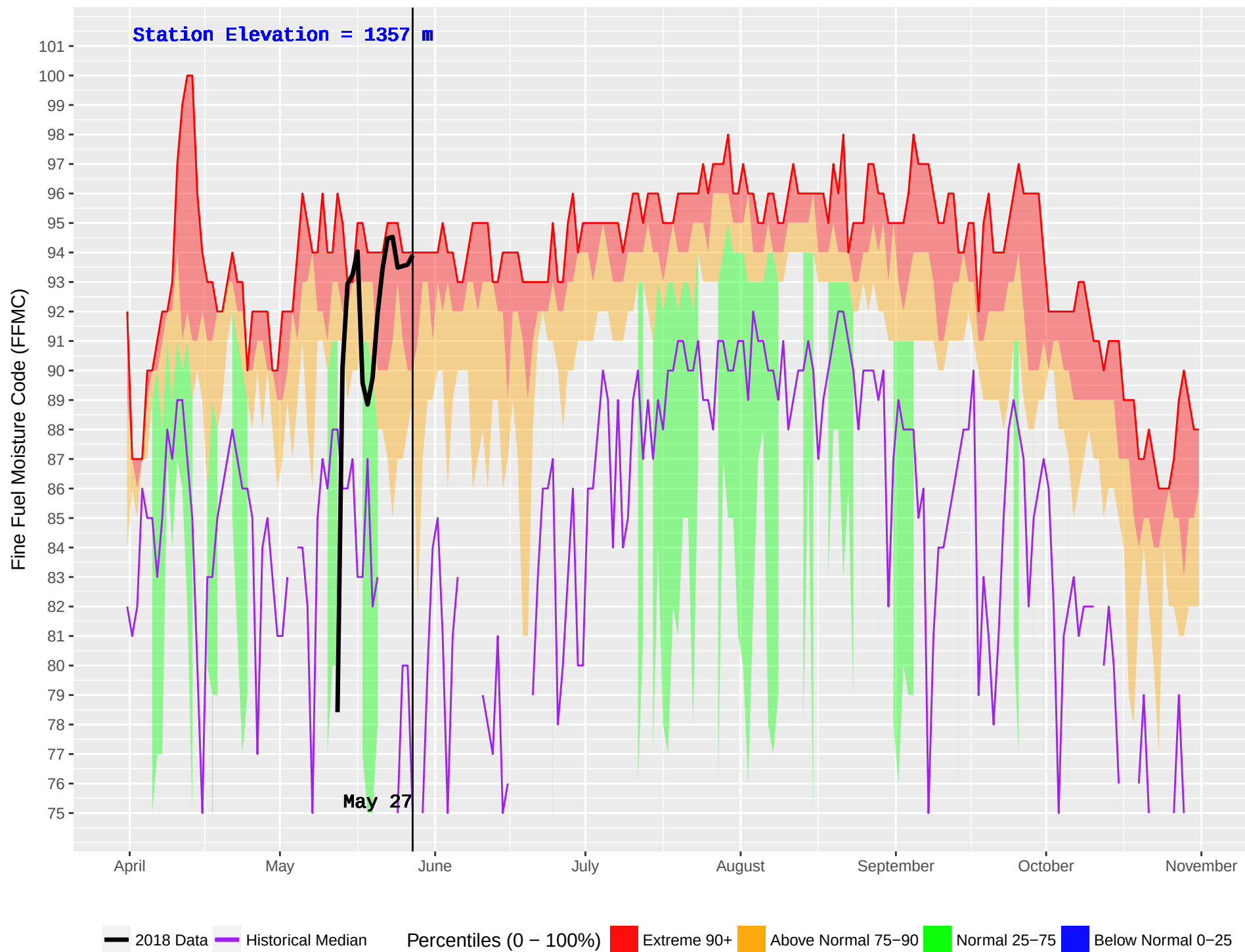
WHITE RIVER (790) : Historical (1989–2016) and Current (2018) Noon Fine Fuel Moisture Code (FFMC)
